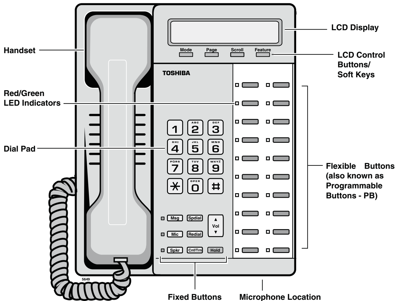
DKT3020-SD Telephone
