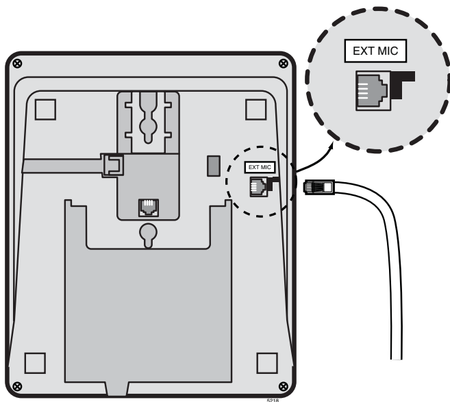
Figure 5 RFDm Plug on DKT2020-FDSP
