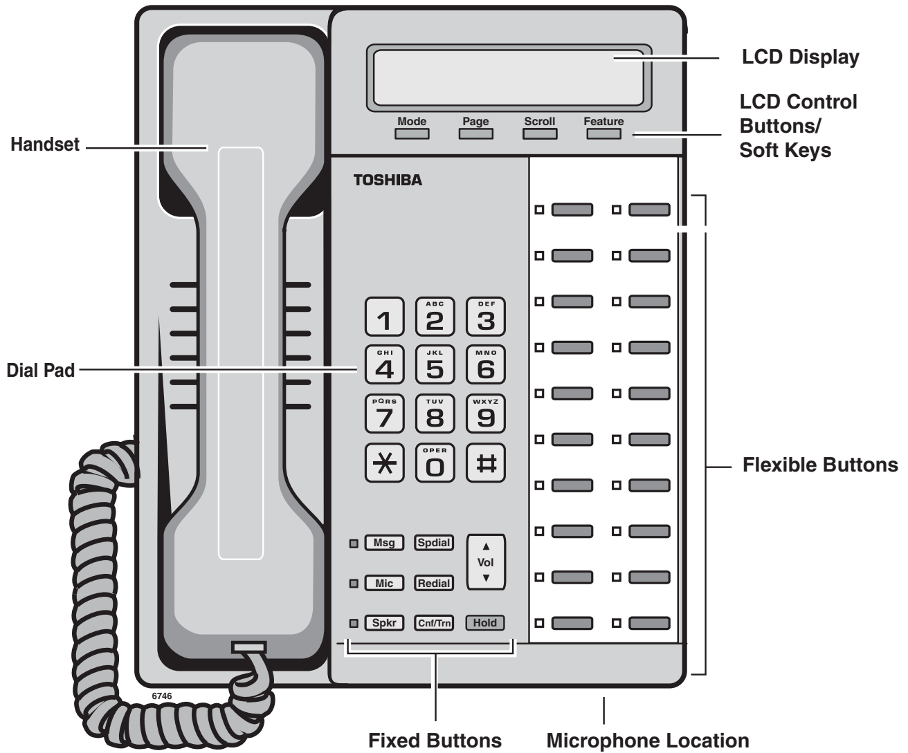
DKT3020-SD Telephone
